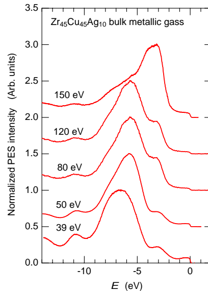
Fig1. h\nu dependence of valence-band PES spectra for Zr_{45}Cu_{45}Ag_{10} bulk metallic glass..
