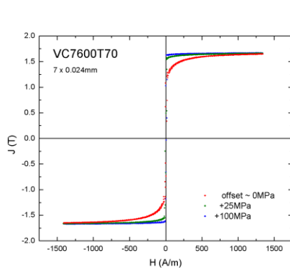
Fig. 1: Stress-dependent ribbon measurement on the narrow-band VC7600T70 sample ( H_{\text{max}} \sim 11000 A/m)
