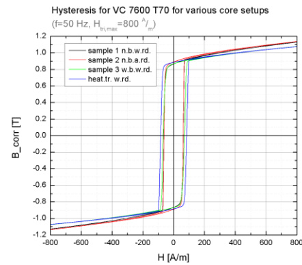
Fig. 2: hysteresis for triangular H-field on VC7600T70 with various core setups
