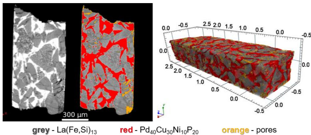
Figure 1. Magnetocaloric composite with Pd-based amorphous matrix.
