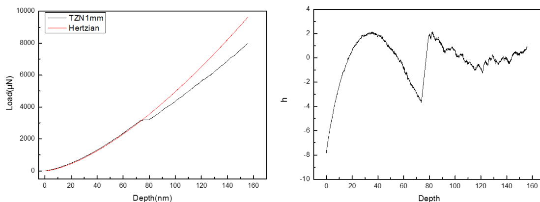
Fig1. Serration behaviour of TiZrNi quasicrystal
