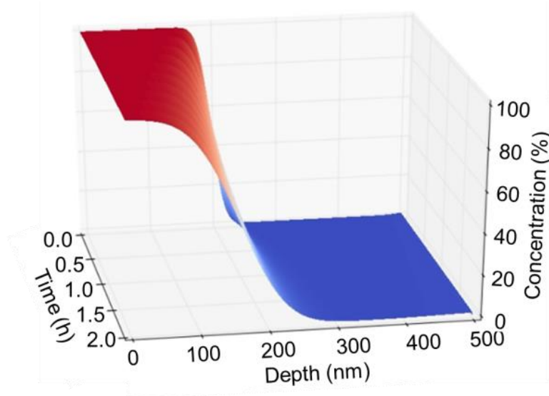
Fig1. Effect of strain on the variation of diffusion profile of Fe in cold-rolled Zr-based bulk metallic glass.
